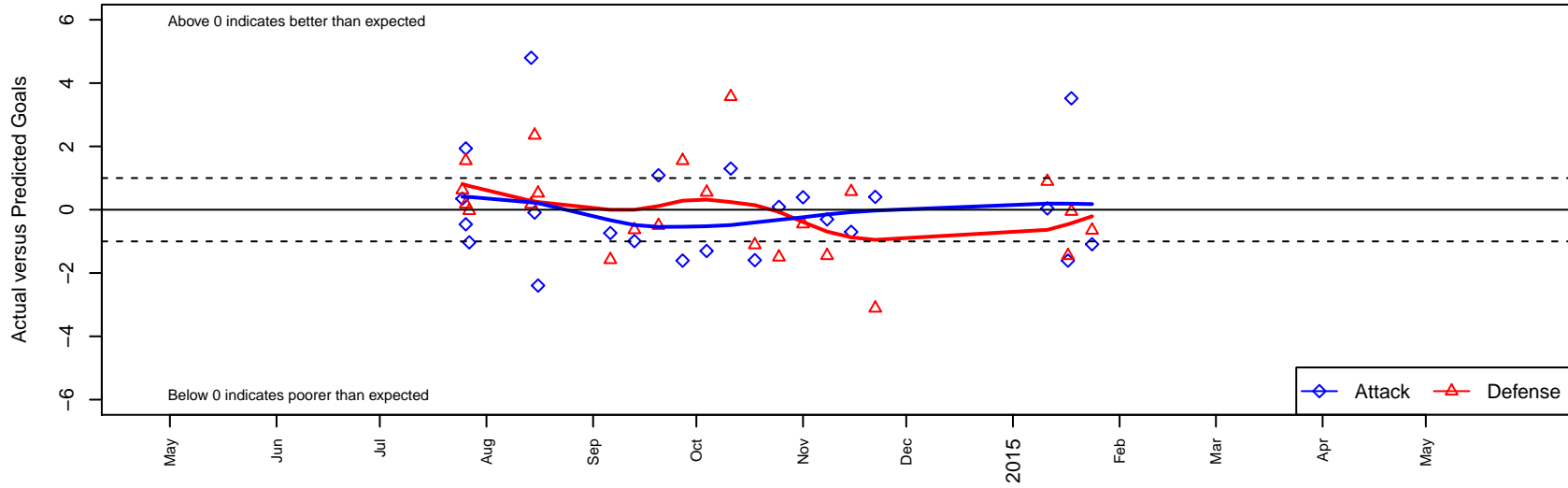
Lake Hills Legends B01 Dots are actual minus expected GF (blue circles) and GA (red triangles). Blue line is smoothed change in attack strength. Red is smoothed change in defense strength.
